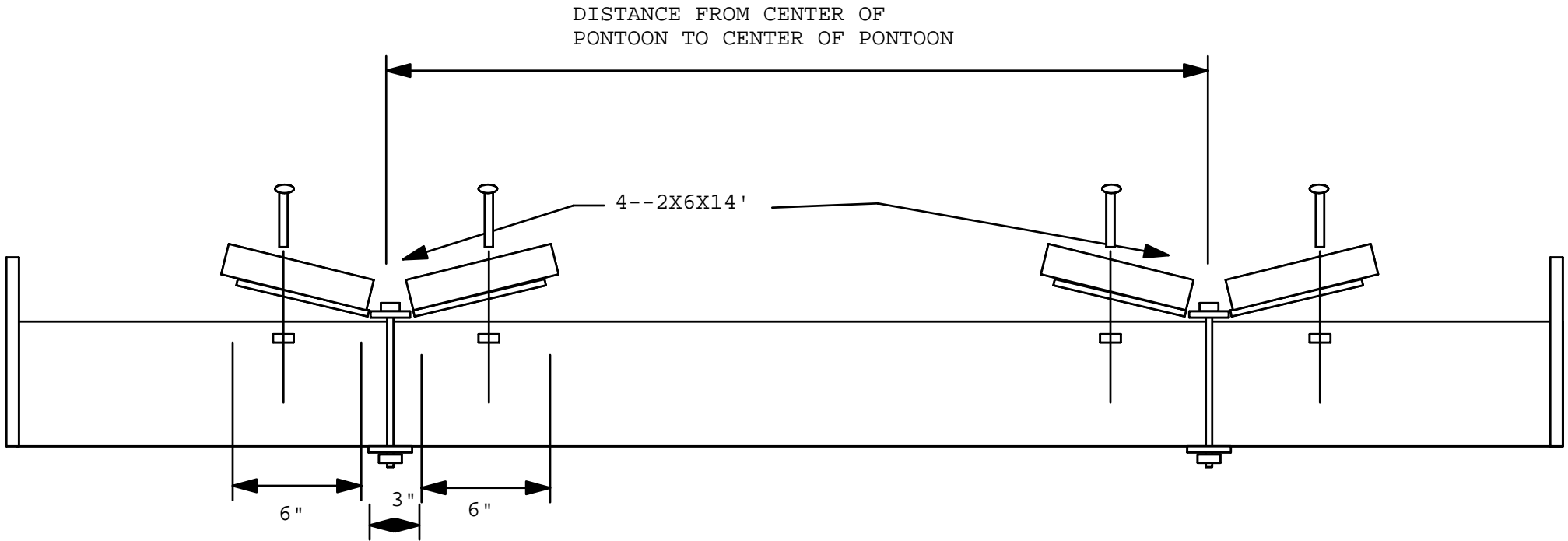
LUNMAR PONTOON CHOCK BRACKETS
